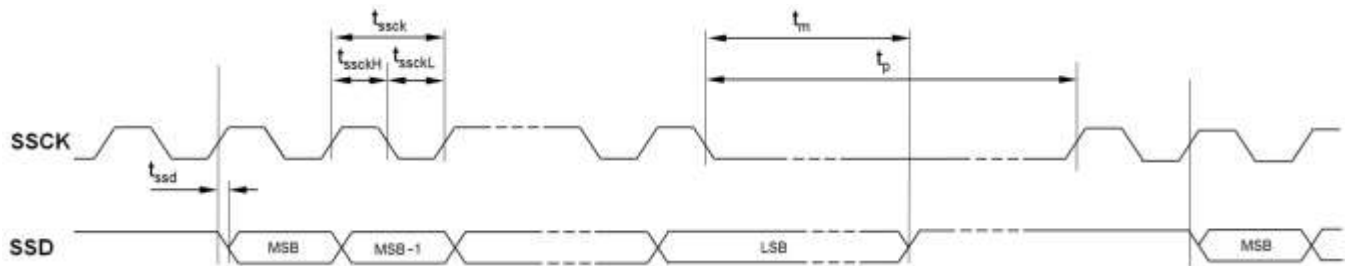
Figure 15: SSI Timing
