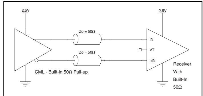
Figure 3D. IN/nIN Input with Built-In 50 \Omega Driven by a CML Driver with Built-In 50 \Omega Pullup
