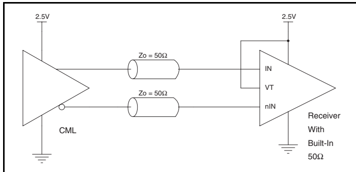
Figure 3C. IN/nIN Input with Built-In 50 \Omega Driven by a CML Driver with Open Collector
