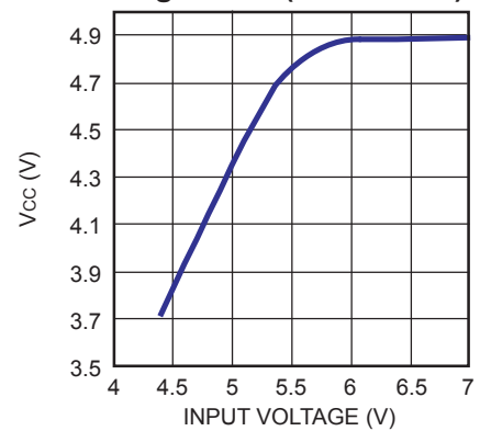
Vcc Regulator Line Regulation ( I_{CC} = 10mA )
