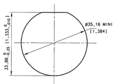
Panel Drilling
