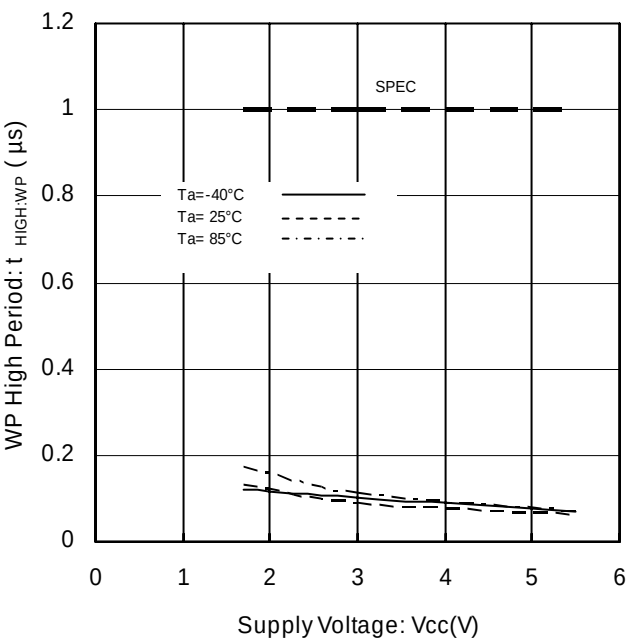
Figure 33. WP High Period vs Supply Voltage
