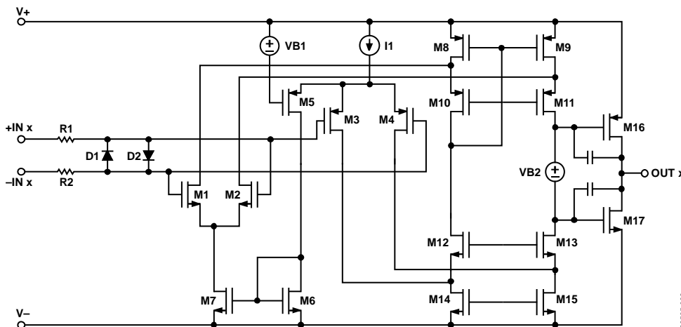
Figure 61. Simplified Schematic
