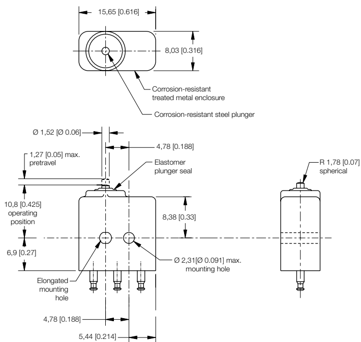
Figure 4. MICRO SWITCH™ XE Dimensions, Solder Terminal
