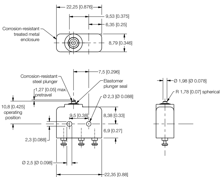
Figure 2. MICRO SWITCH™ SE Dimensions, Solder Terminal
