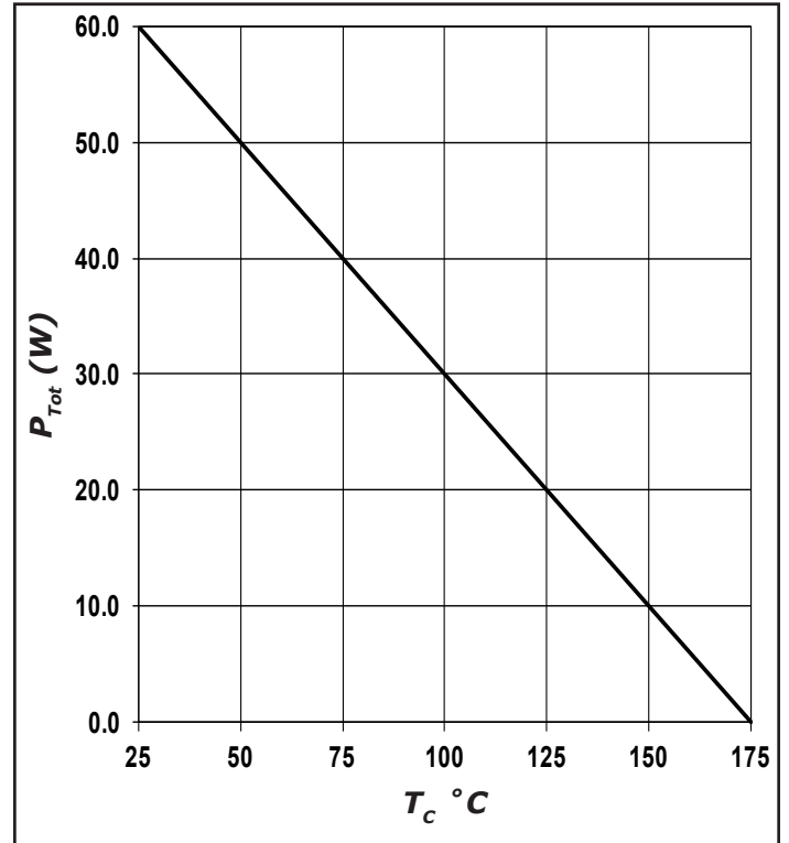
Figure 4. Power Derating
