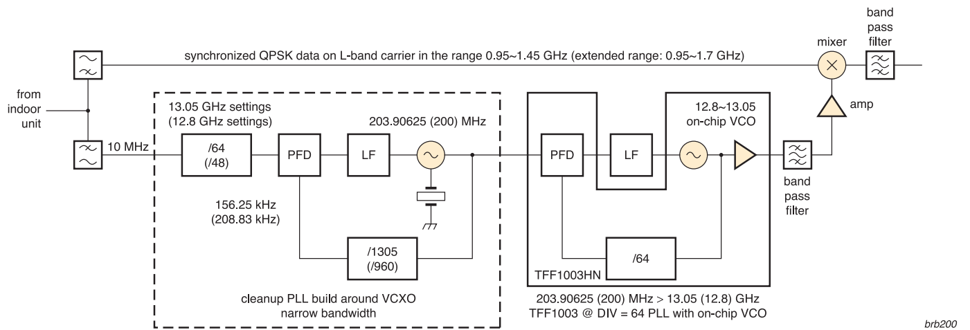
Complete LO generator for linear BUC with TFF1003HN
