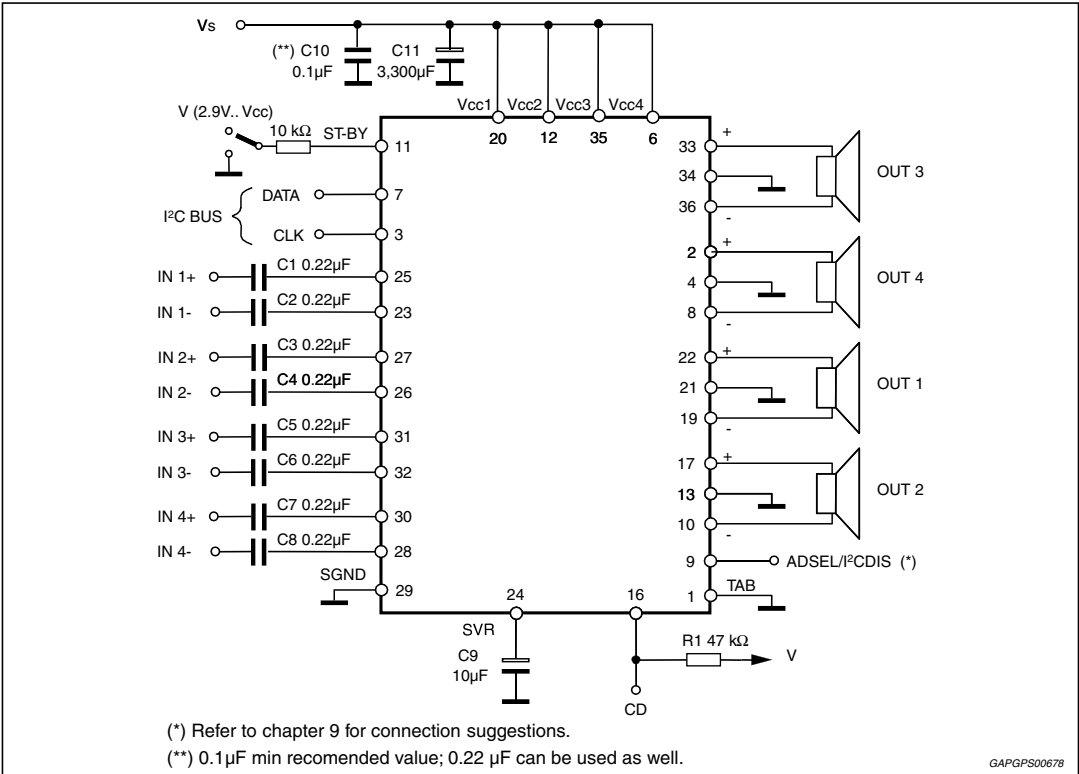
Figure 2. Application circuit
