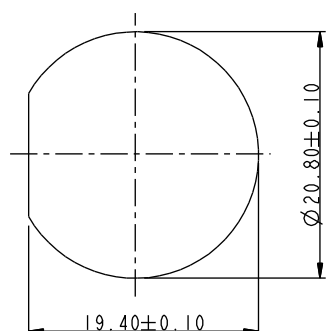
Recommended Panel Cut-out Rear View
