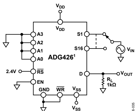
Figure 35. Off Isolation
