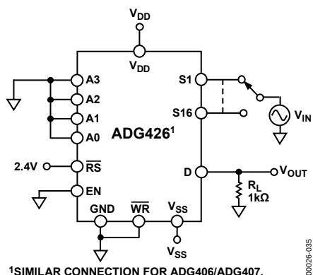
Figure 35. Off Isolation
