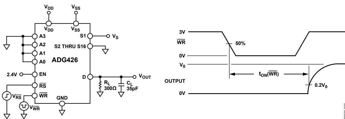
Figure 32. Write Turn-On Time, t ON (WR)
