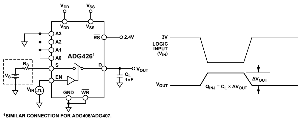
Figure 34. Charge Injection
