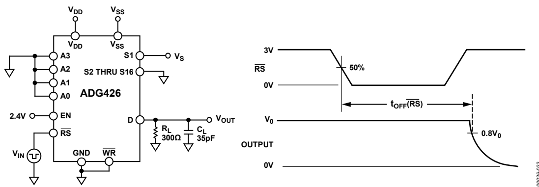
Figure 33. Reset Turn-Off Time, t OFF (RS)
