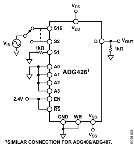
Figure 36. Crosstalk
