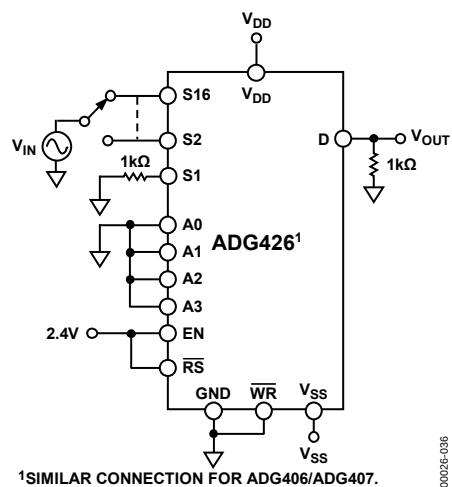
Figure 36. Crosstalk
