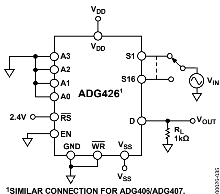
Figure 35. Off Isolation
