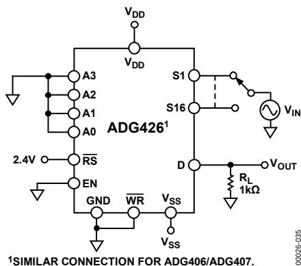
Figure 35. Off Isolation
