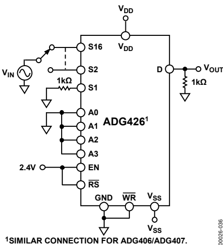
Figure 36. Crosstalk
