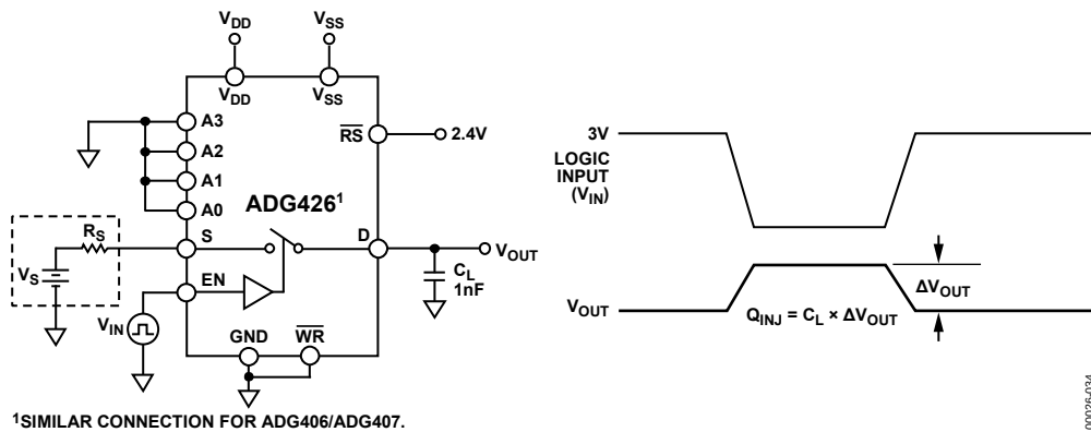
Figure 34. Charge Injection
