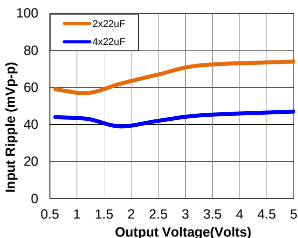
Figure 37. Input ripple voltage for various output voltages with 2x22 \mu F or 4x22 \mu F ceramic capacitors at the input (2 × 6A load). Input voltage is 12V. Scope BW: 20MHz
