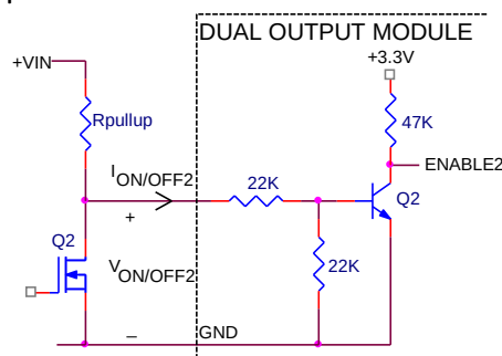
Figure 40. Circuit configuration for using negative On/Off logic.
