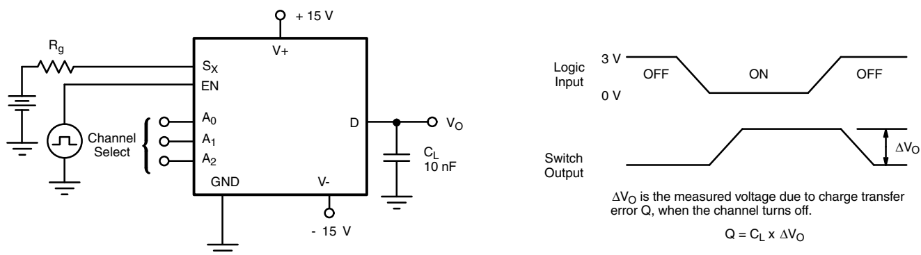
Fig. 5 - Charge Injection
