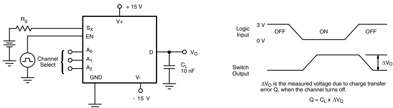
Fig. 5 - Charge Injection
