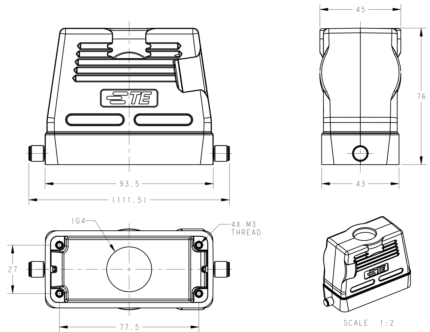
TYPE 4: HIGH CONSTRUCTION, TOP ENTRY
