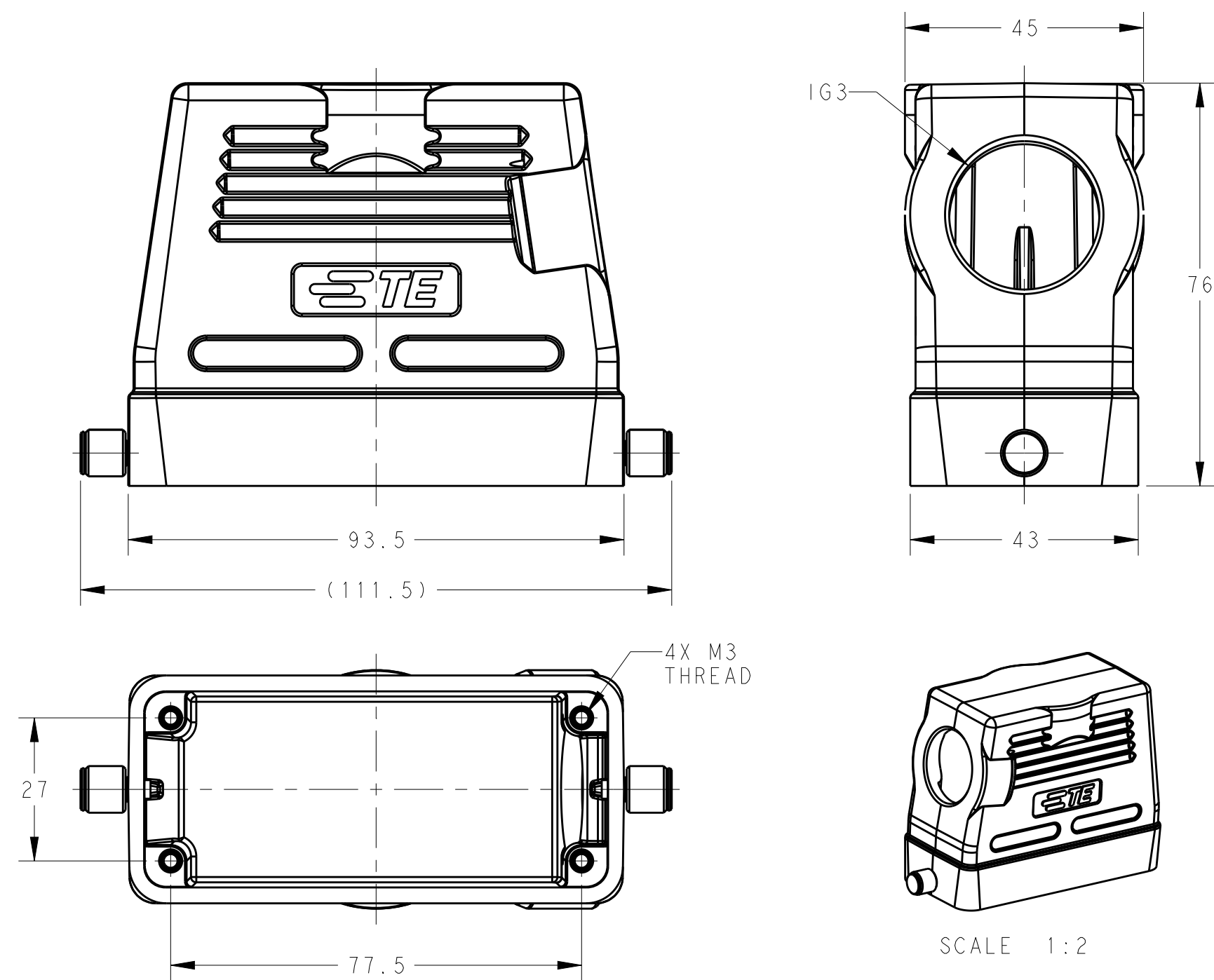
TYPE 3: HIGH CONSTRUCTION, SIDE ENTRY
