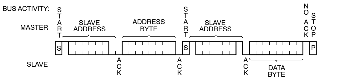
Figure 11. Selective Read Sequence
