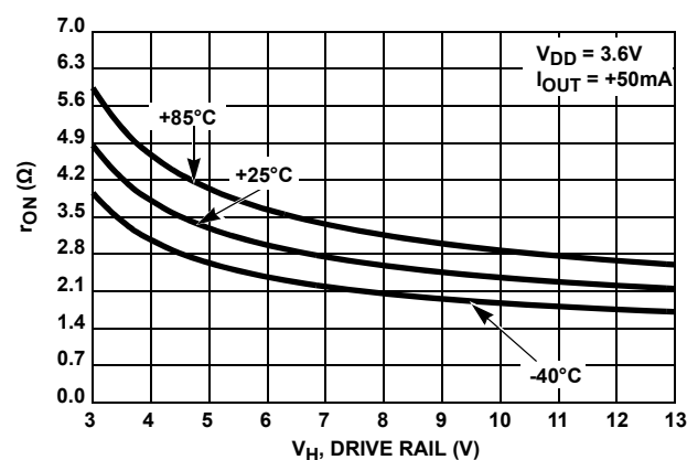
FIGURE 5. DRIVER r_{ON} vs V_H VOLTAGE (SINKING CURRENT)
