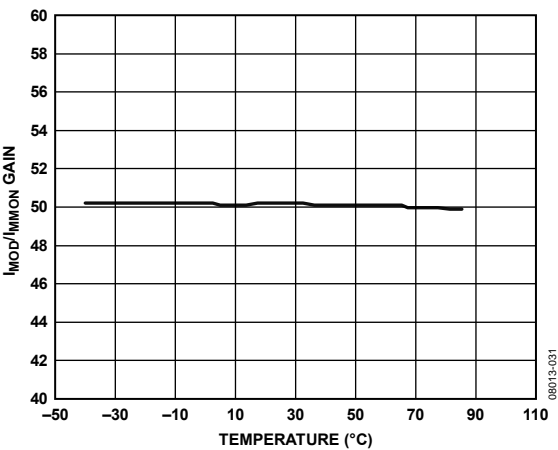
Figure 15. I_{MOD}/I_{MMON} Gain vs. Temperature, I_{MOD} = 30\text{ mA}
