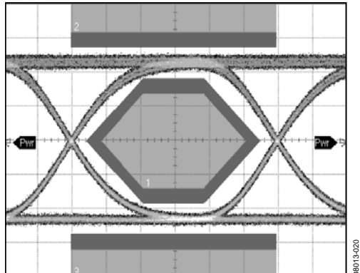
Figure 20. Optical Eye 155 Mbps, 1.078 ns/DIV, PRBS 2^{31} - 1 , PAV = -4.5 dBm, ER = 9 dB, Mask Margin 50%
