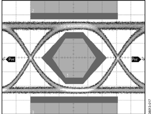
Figure 19. Optical Eye 622 Mbps, 264 ps/DIV, PRBS 2^{31} - 1 , PAV = -4.5 dBm, ER = 9 dB, Mask Margin 50%
