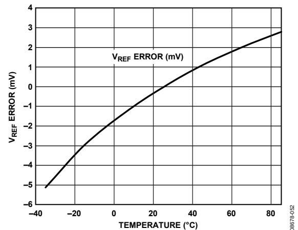
Figure 44. Typical VREF Drift
