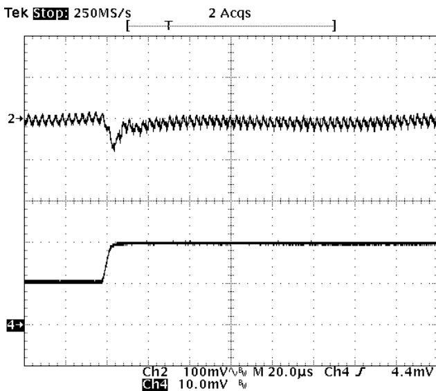
Fig-3.3V-6: Output voltage response for V_{out}=3.3V to positive load current step-change from 5A to 10A with slew rate of 5A/us at V_{in}=12V . C_o=47\mu F \times 2 ceramic. Top trace: output voltage (100mV/div.) Bottom trace: load current (5A/div.) Time scale: 20us/div.
