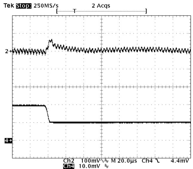
Fig-3.3V-7: Output voltage response for V_{out}=3.3V to negative load current step change from 10A to 5A with slew rate of -5A/us at V_{in}=12V . C_o=47\mu F \times 2 ceramic. Top trace: output voltage (100mV/div.) Bottom trace: load current (5A/div.) Time scale: 20us/div.
