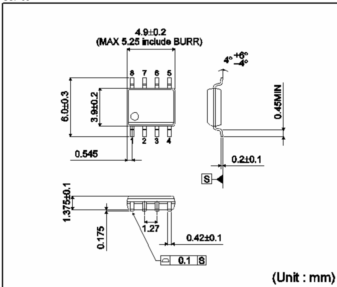
SOP-J8
