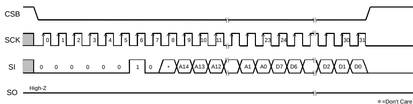
Figure 34. Write command
