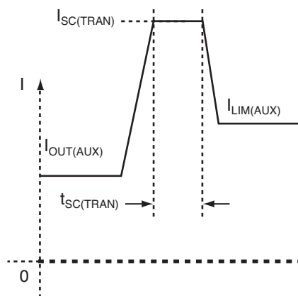
Figure 4. VAUX Current Limit Response Timing
