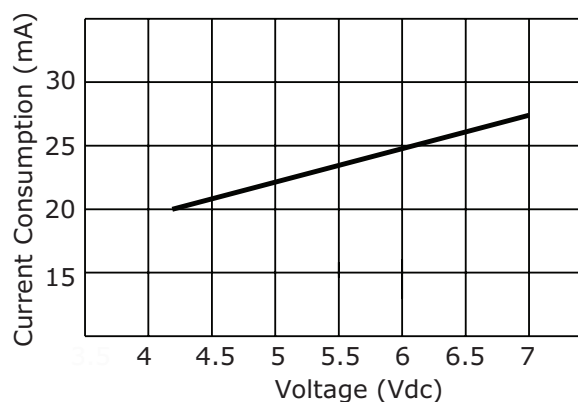
Voltage vs. Current Consumption at 25°C
