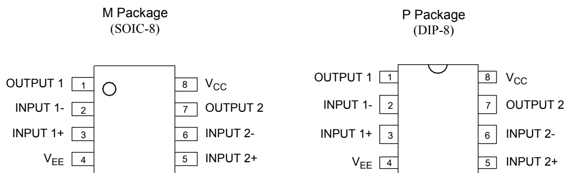
Figure 2. Pin Configuration of AZ4558C (Top View)
