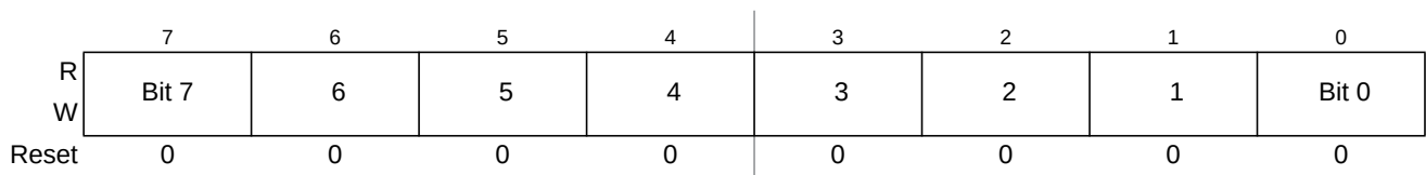
Figure 13-12. PWM Scale B Register (PWMSCLB)
