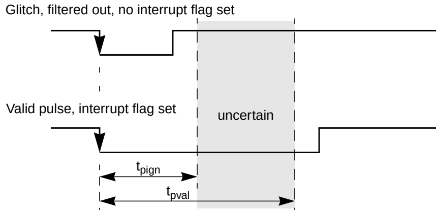
Figure 2-95. Interrupt Glitch Filter on Port T,S,R, and AD(PPS=0)
