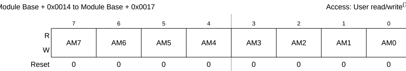
Figure 11-22. MSCAN Identifier Mask Registers (First Bank) — CANIDMR0–CANIDMR3
