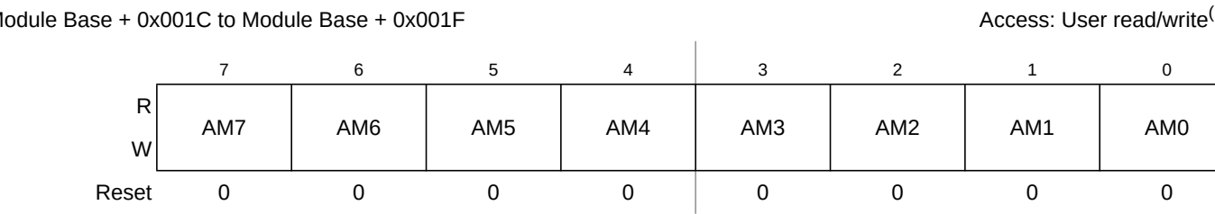
Figure 11-23. MSCAN Identifier Mask Registers (Second Bank) — CANIDMR4–CANIDMR7
