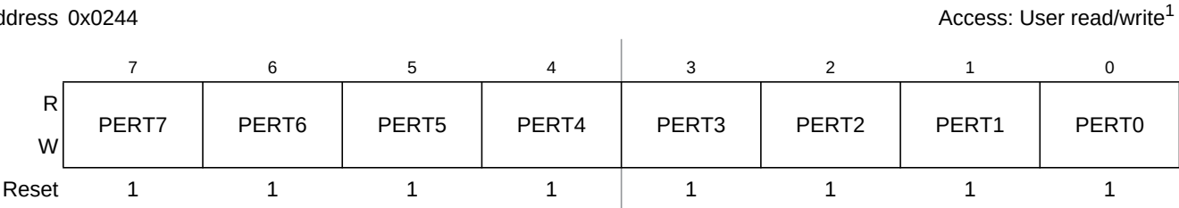
Figure 2-16. Port T Pull Device Enable Register (PERT)
