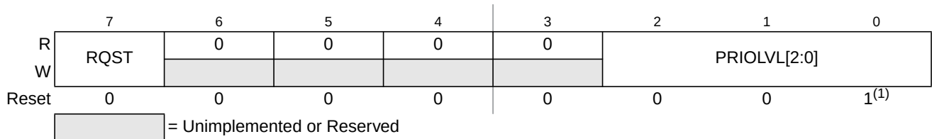
Figure 4-6. Interrupt Request Configuration Data Register 0 (INT_CFDATA0)
