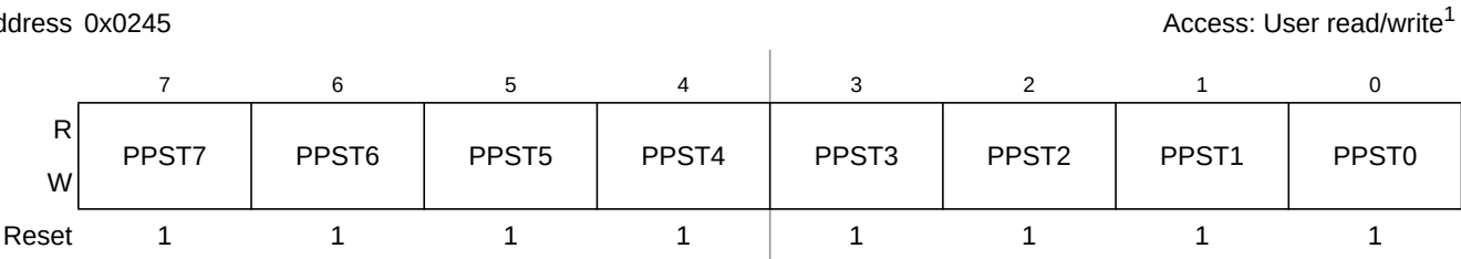
Figure 2-17. Port T Polarity Select Register (PPST)
