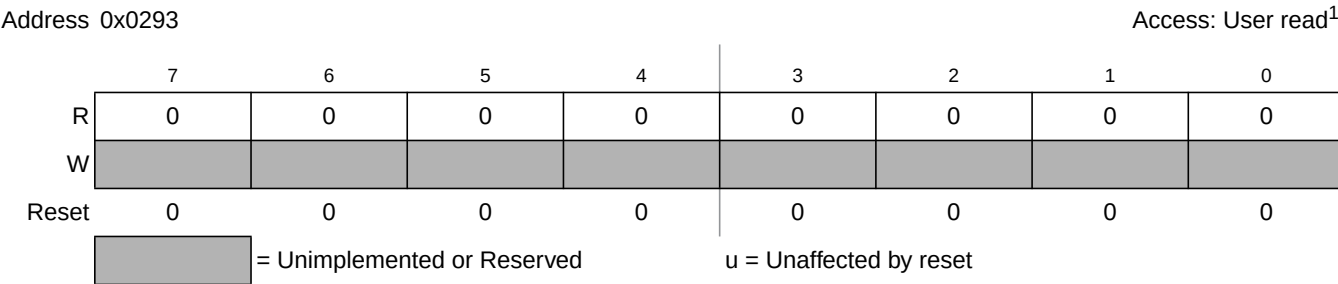
Figure 2-81. PIM Reserved Registers
