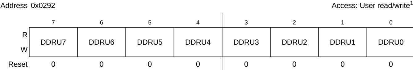
Figure 2-80. Port U Data Direction Register (DDRU)
