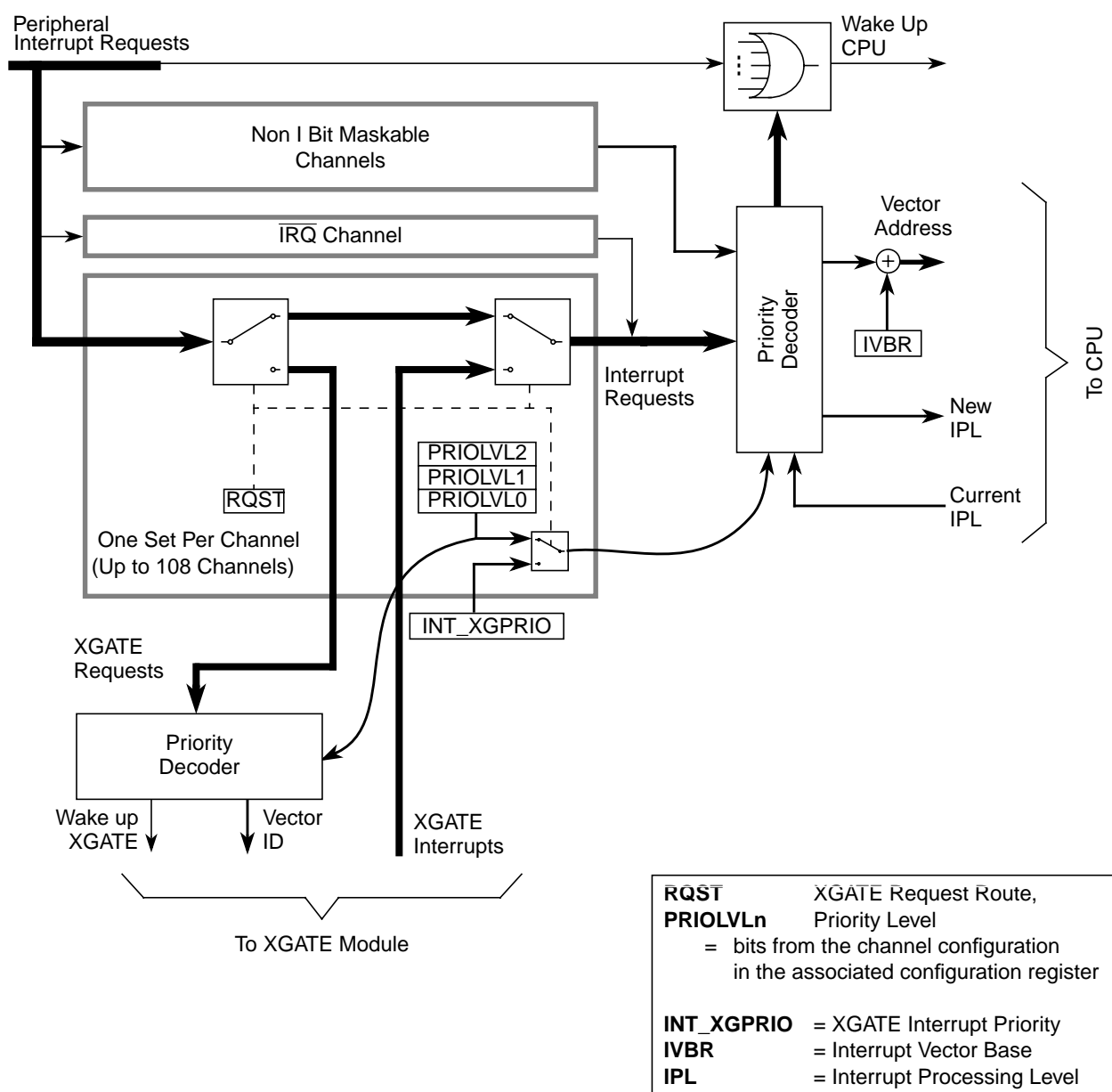
Figure 4-1. XINT Block Diagram
