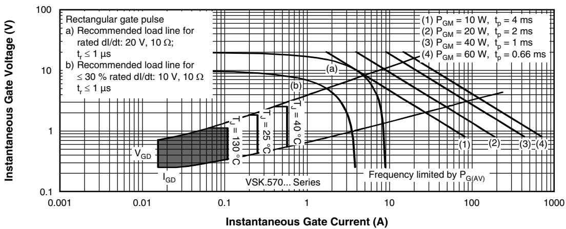
Fig. 10 - Gate Characteristics
