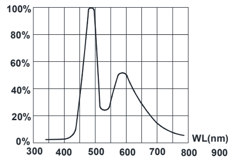
FIG.4 RELATIVE LUMINOUS INTENSITY VS. WAVELENGTH. 50% Power Angle : 120°
