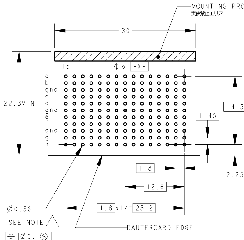
RECOMMENDED PC BOARD LAYOUT VIEWED FROM CONNETOR SIDE SCALE 2:1
