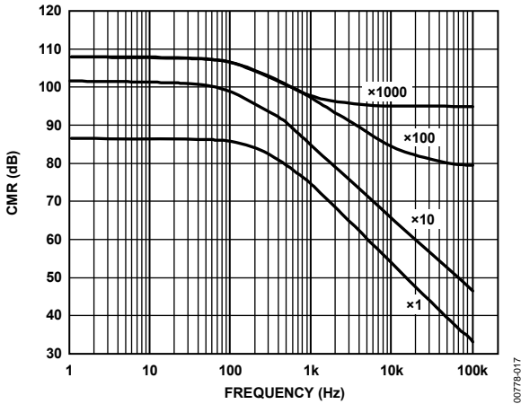
Figure 17. CMR vs. Frequency, = 5 V_S, 0 V_{REF} , V_{REF} = 2.5 V
