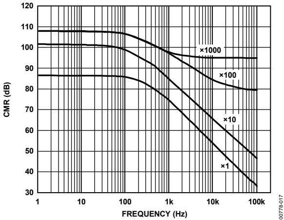
Figure 17. CMR vs. Frequency, \pm 5 V_S , 0 V_{S_2} , V_{REF} = 2.5 V
