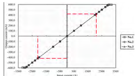
Saturation Characteristics
