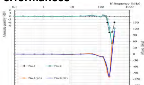
Frequency Characteristics
