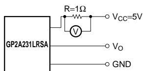
Fig.1 Test Condition for Peak Pulse Value I CCP
