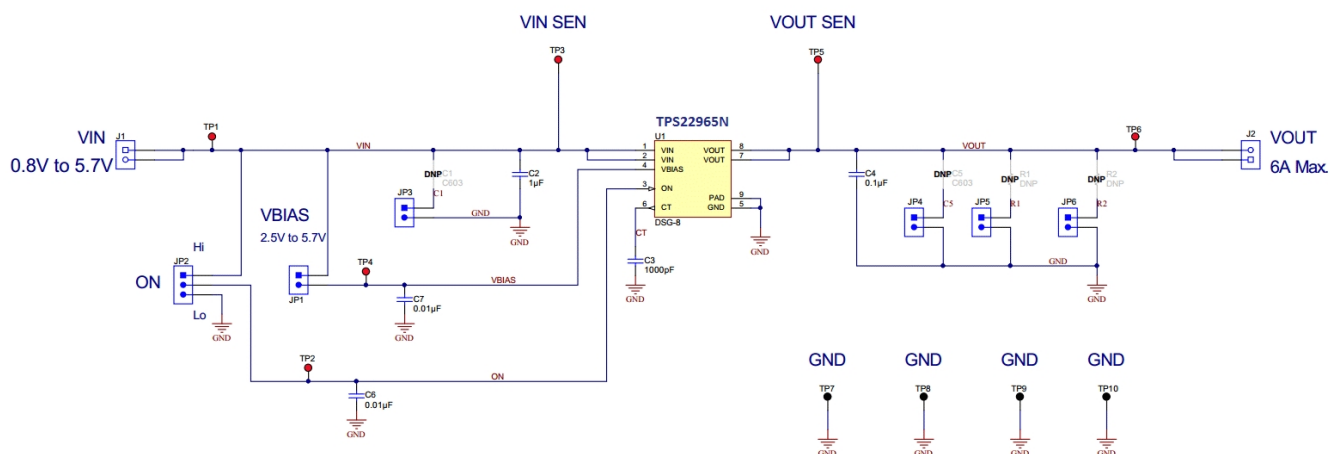
Figure 2. TPS22965NEVM Schematic
