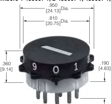
thumbwheel Part Number 435097-1 (shown) Part Number 435097-2 (with numbers 1-10)
