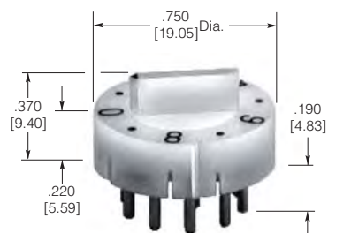
bar type knob Part Number 2-435097-1
