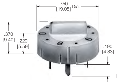
bar type knob Part Number 1-435123-1
