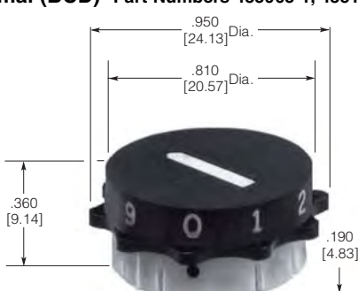
thumbwheel Part Number 435128-1
