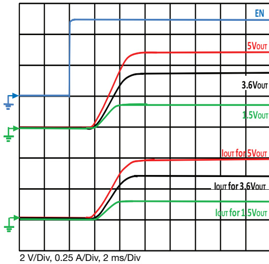
Figure 25 - Typical Turn-on Delay, Rise Time C_{OUT} = 200 \mu F , C_{IN} = 4.7 \mu F , R_{OUT} = 10 \Omega
