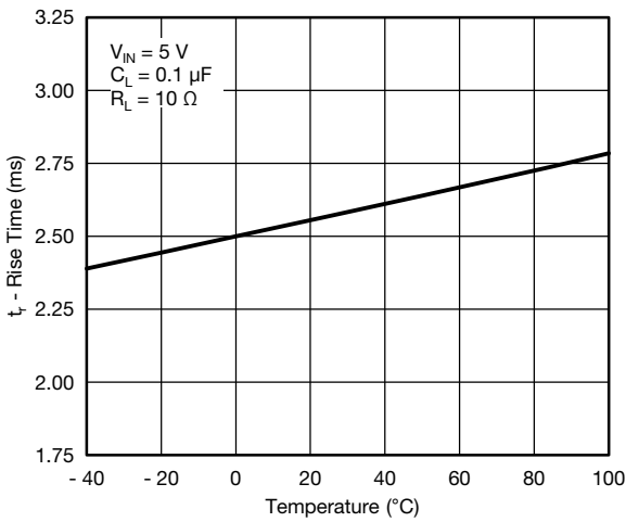
Figure 15 - Rise Time vs. Temperature
