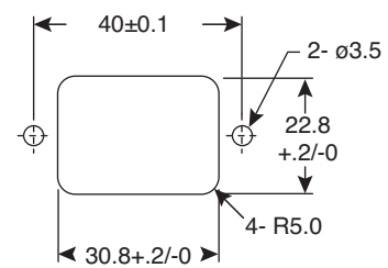
Rear Mounting
