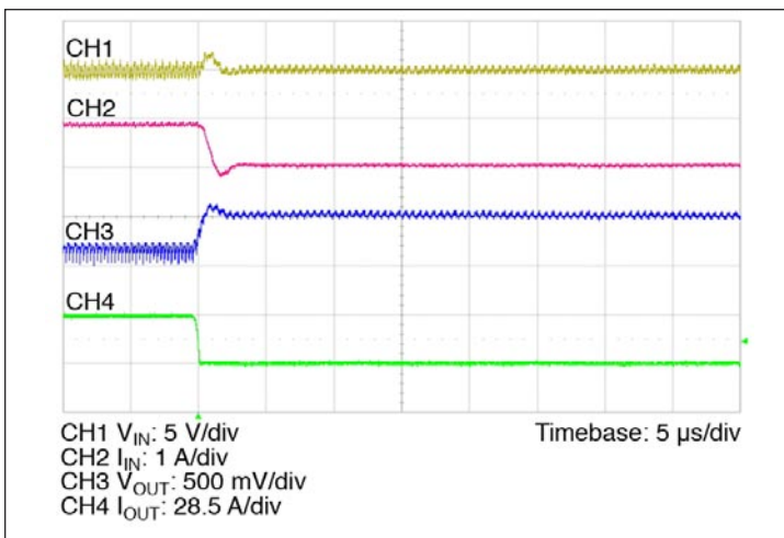
Figure 12 — 28.5 A–0 A transient response: C_{IN} = 2.2 \mu F , no external C_{OUT}
