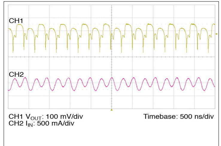
Figure 9 — Full load ripple, 2.2 \mu F C_{IN} ; No external C_{OUT} . Board mounted module, scope setting : 20 MHz analog BW
