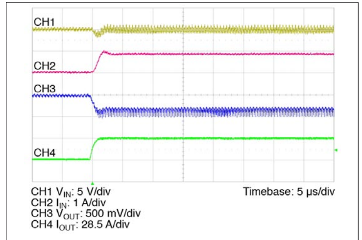
Figure 11 — 0 A–28.5 A transient response: C_{IN} = 2.2 \mu F , no external C_{OUT}
