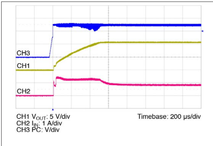
Figure 10 — Start up from application of PC; V_{IN} pre-applied C_{OUT} = 1200 \mu F
