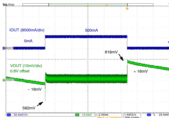
Figure 17. Load Transient, 3.8 V IN , 0.6 V OUT , 0–500 mA, 100 ns Edge, 47 μF C OUT
