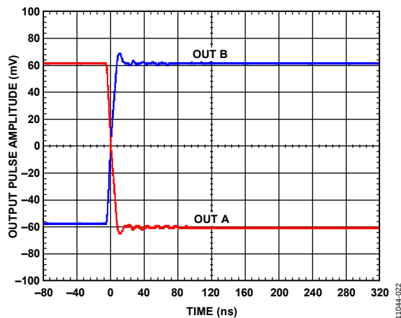
Figure 6. Small Signal Output Transient Response, Normalized to 0 V, 10 ns Rise Time, 10 ns Fall Time, 1 \mu s Pulse Width, 10% Duty Cycle
