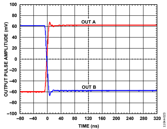
Figure 9. Small Signal Output Transient Response, Normalized to 0 V, 10 ns Rise Time, 10 ns Fall Time, 1 \mu s Pulse Width, 10% Duty Cycle
