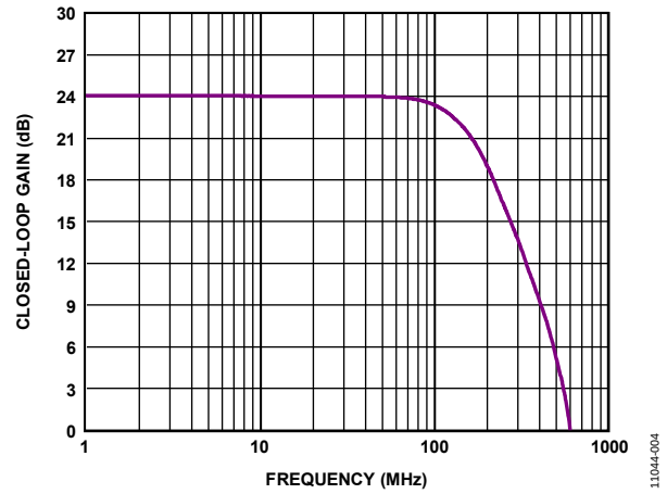
Figure 7. Large Signal Differential Frequency Response, Gain = +16 V/V, Differential V_{OUT} = 5 V_{p-p}
