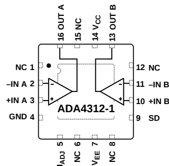
Figure 1. Thermally Enhanced, 4 mm × 4 mm, 16-Lead LFCSP_WQ
