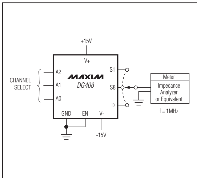
Figure 8. Source/Drain Capacitance
