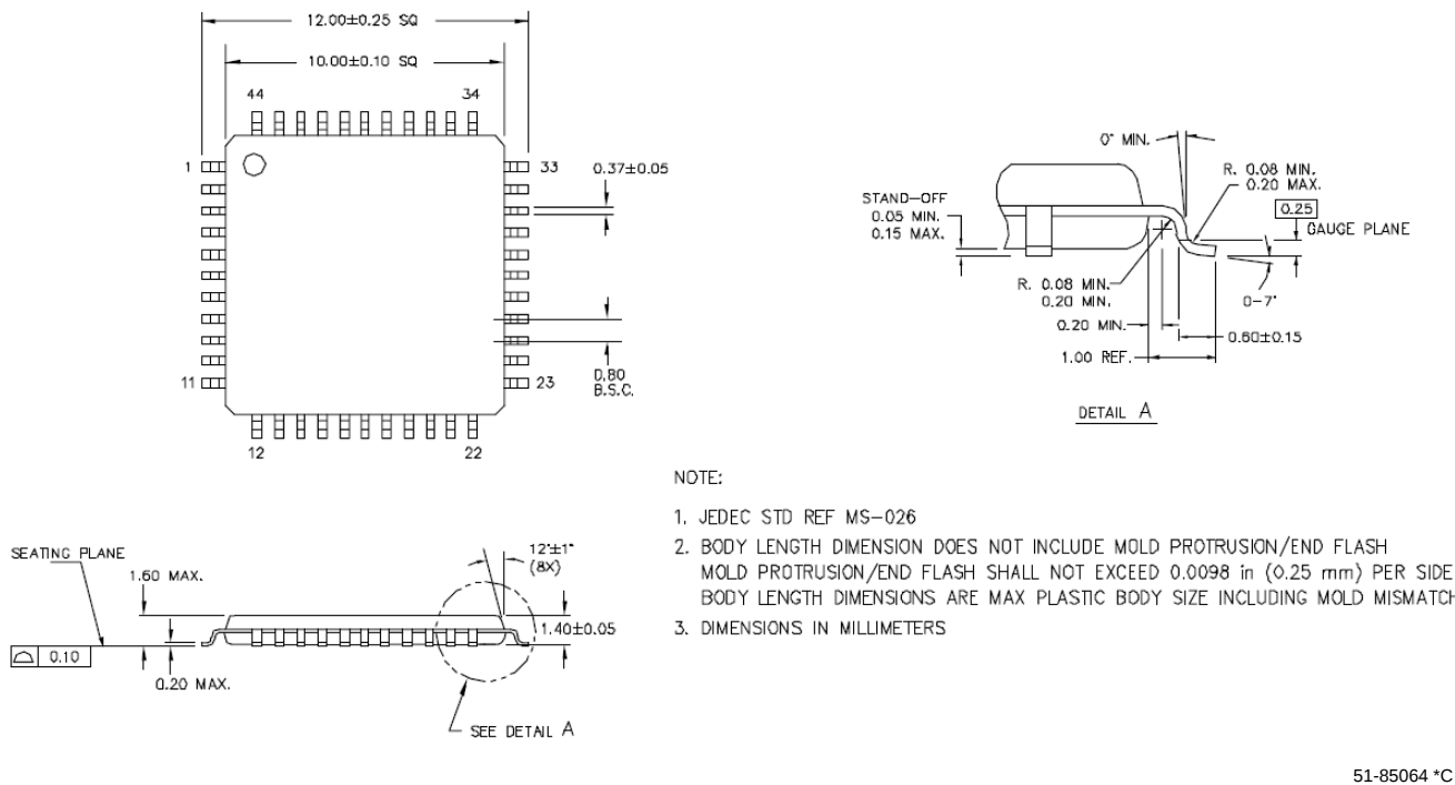
Figure 4-7. 44-Lead TQFP
