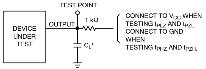
Figure 6. Test Circuit
